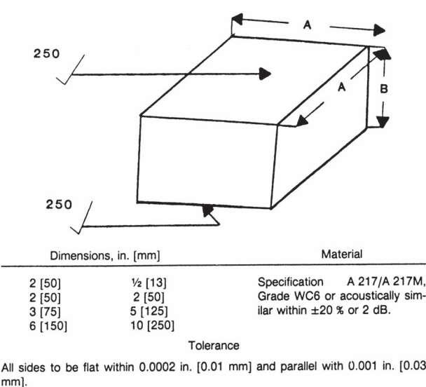
FIG. 3 CALIBRATION BLOCKS
