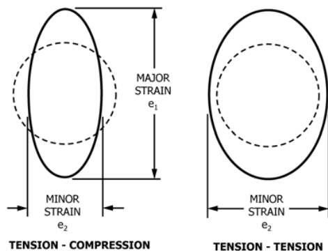
FIG. X4.2 Major and Minor Strain Axes
